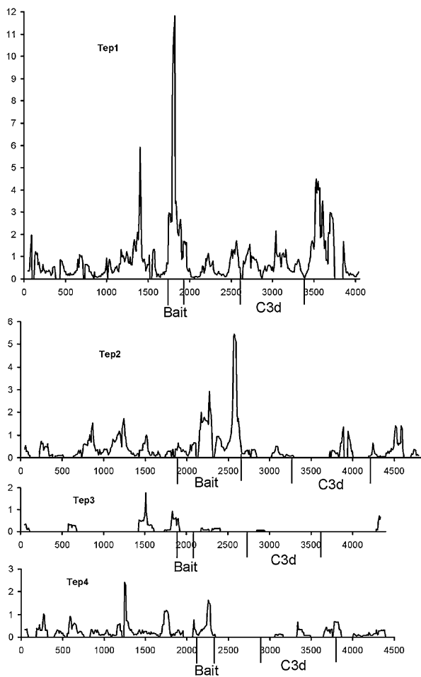
Fig. 2. Sliding window analysis of the K_a/K_s ratio along the entire coding sequence of the four Tep genes in D. simulans and D. melanogaster . The bait-like and C3d-like regions are marked. Window size = 100 bp; step size = 1 bp; K_a/K_s ratio estimated following Nei and Gojobori (1986).
